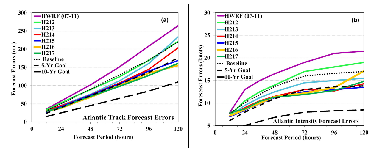
Figure 1: HWRF improvements in forecast track (a) and intensity (b) error for the Atlantic Basin from 2007-2011 to 2017 under HFIP are shown. Seasons for which models were run are depicted on each line. Note that some samples (years) are not homogeneous between models.
