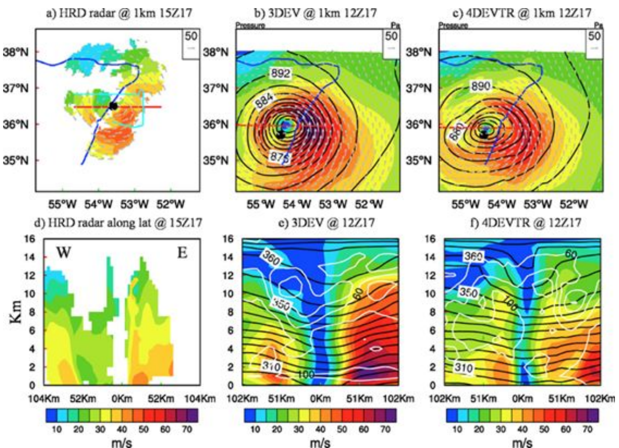
Figure 10. A comparison of observations and analyses of Hurricane Edouard in terms of (a-c) Horizontal plots at 1-km height and (d-f) vertical cross sections through the center on 17 September 2014. All horizontal plots show wind speed (filled) overlain with wind vectors, while the analyses also show pressure (black contour) and relative humidity (white contour). The blue line in (a-c) denotes the flight track when TDR data is available between 1258-1417 UTC, and the turquoise line in (a) denotes the flight track when TDR data is available between 1617-1708 UTC. Due to the data distribution, the HRD radar composite is valid at 1500 UTC 17 September 2014, while the analyses are at 1200 UTC. Figure taken from Lu et al. (2017).
